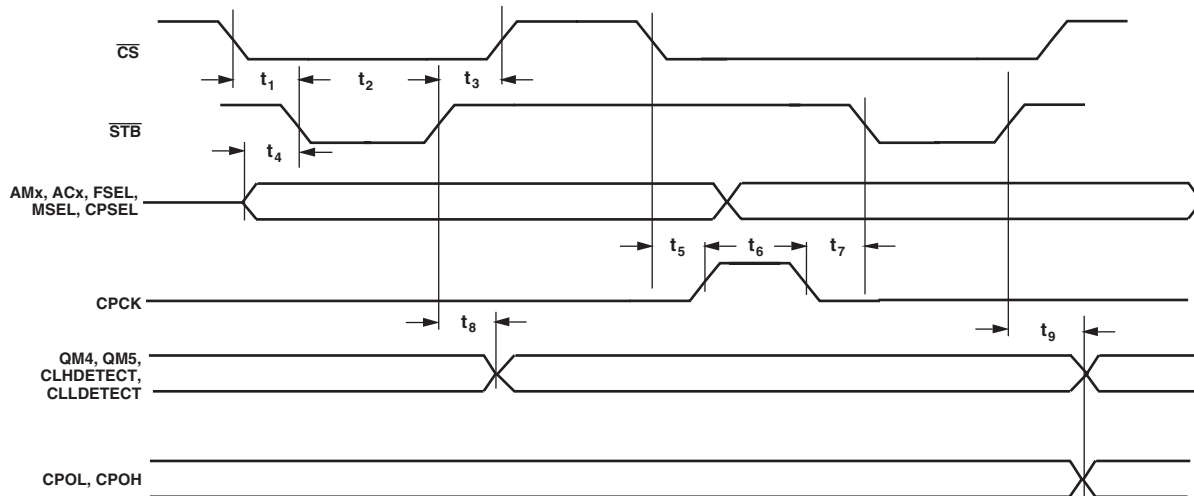
Figure 1. Timing Diagram
