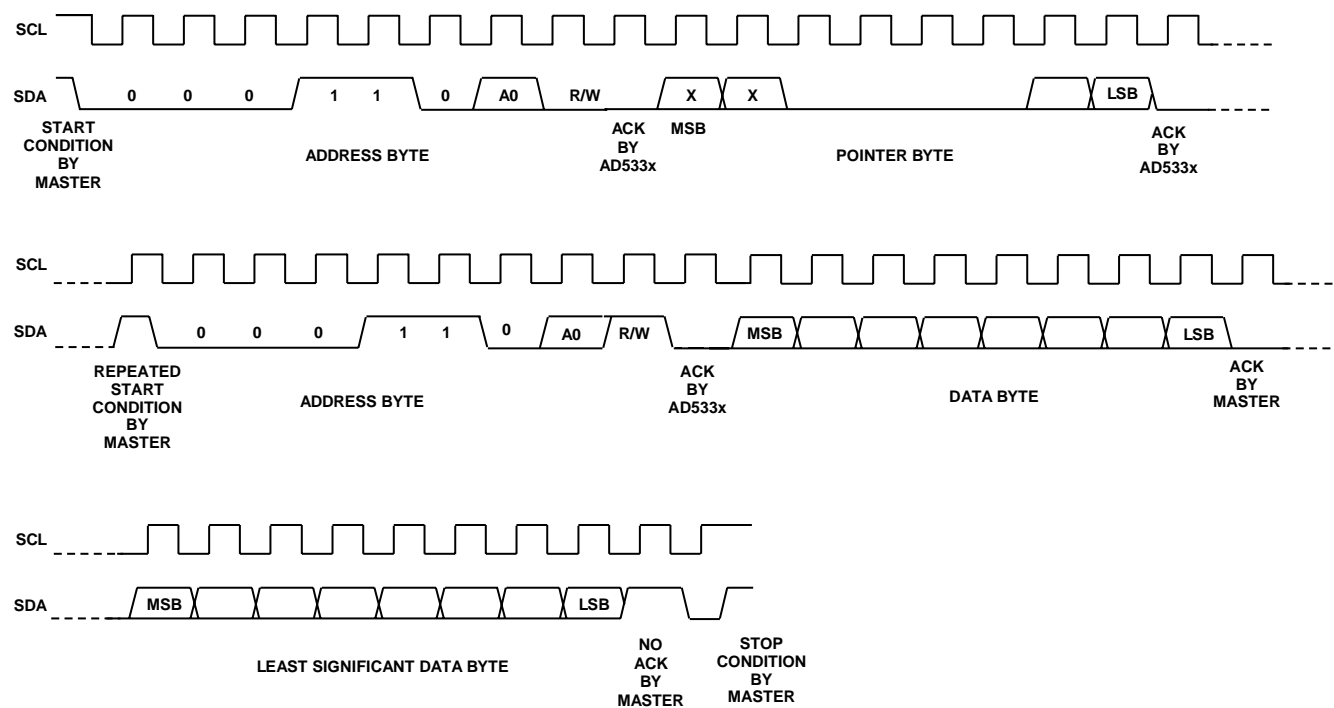
Figure 34. Read Sequence
