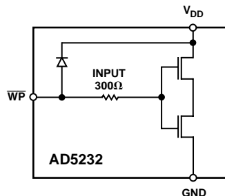
Figure 4b. Equivalent \overline{\text{WP}} Input Protection
