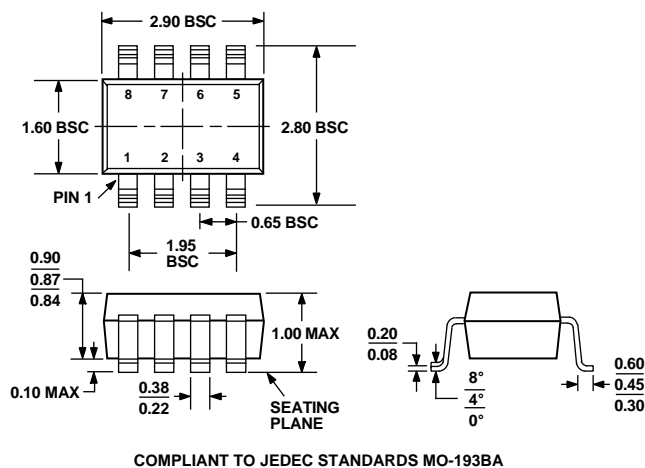
Figure 48. 8-Lead Small Outline Transistor Package TSOT-8 [Thin SOT-23-8] (UJ-8) Dimensions shown in millimeters
