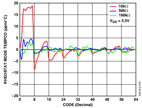
Figure 15. Rheostat Mode Tempco \Delta R_W/\Delta T vs. Code
