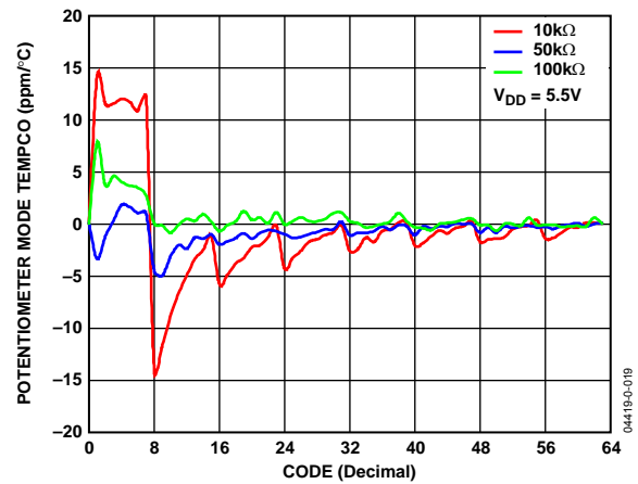
Figure 16. Potentiometer Mode Tempco \Delta R_W/\Delta T vs. Code
