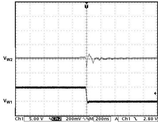
Figure 23. Digital Crosstalk
