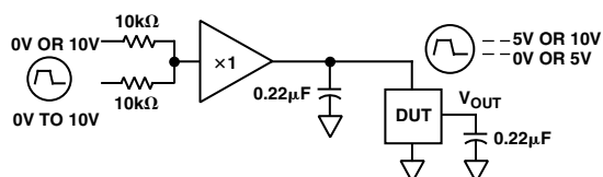
Figure 12a. Turn-On/Transient Response Test Circuit
