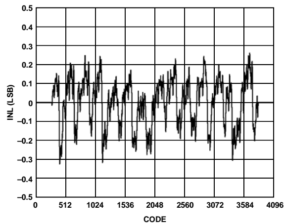
Figure 14. Typical INL
