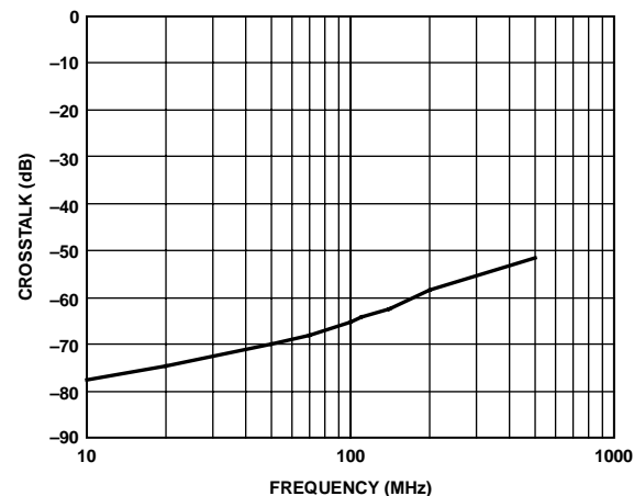
Figure 9. Typical Crosstalk
