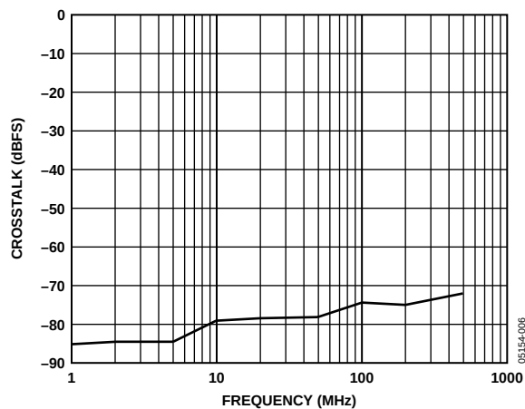
Figure 5. Typical Crosstalk
