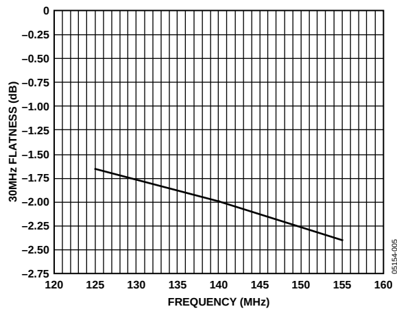
Figure 4. Gain Flatness f_{IN} = 125 MHz to 155 MHz
