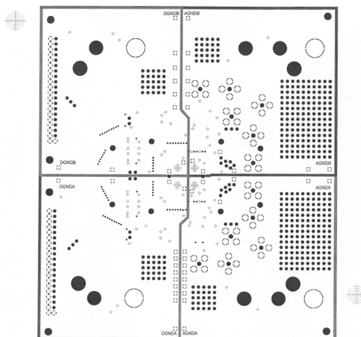
Figure 11d. GND2
