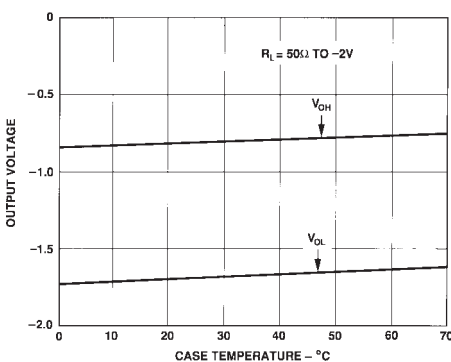
Figure 14. Output Levels vs. Temperature
