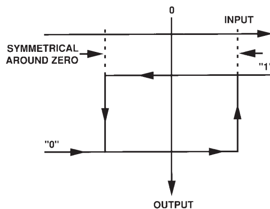
Figure 30. Hysteresis
