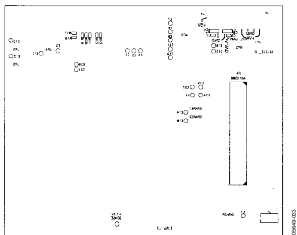
Figure 33. Top Silkscreen
