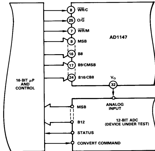
Figure 7. ADC Testing
