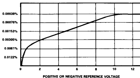
Figure 5. Typical Differential Linearity vs. External Reference Voltage
