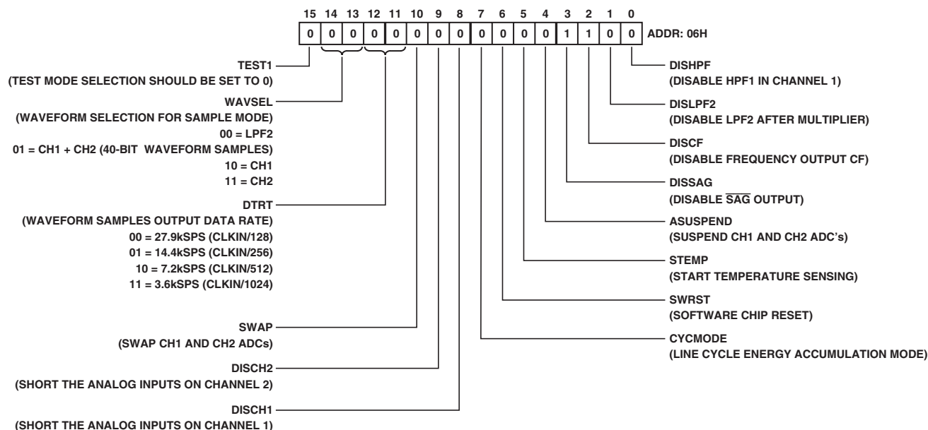
Figure 48. Mode Register
