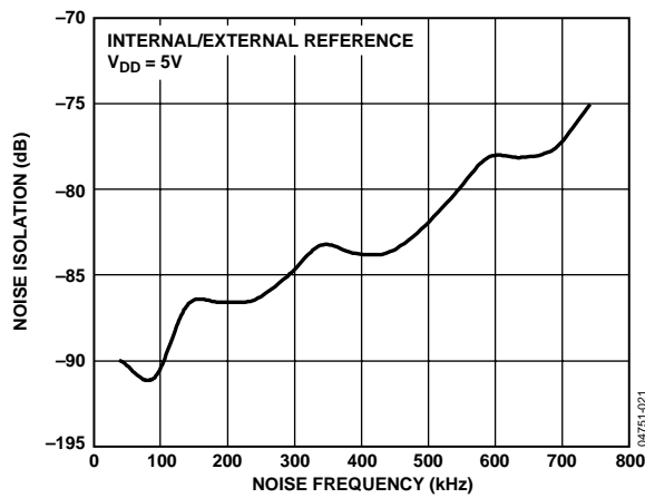
Figure 4. AD7938-6 Channel-to-Channel Isolation
