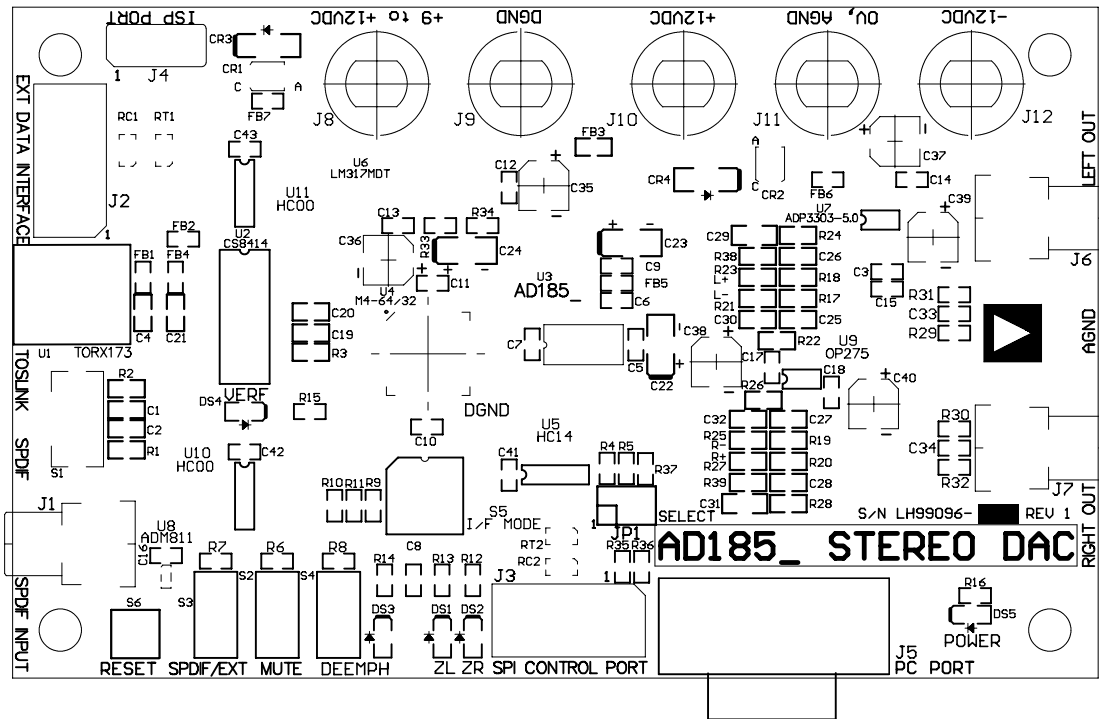
Figure 3. Silk Screen
