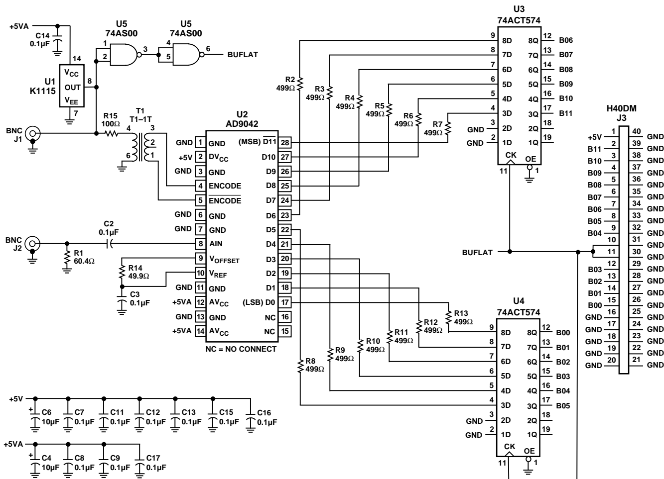
Figure 37. AD9042D/PCB Schematic
