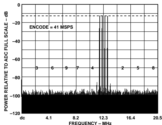
Figure 56. Multitone Performance
