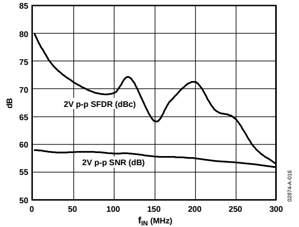
Figure 19. AD9215-80 SNR/SFDR vs. f_{\text{IN}} , A_{\text{IN}} = -0.5 \text{ dBFS} , f_{\text{SAMPLE}} = 80 \text{ MSPS}
