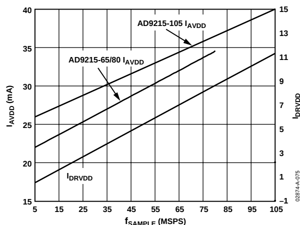
Figure 35. Supply Current vs. f_{\text{SAMPLE}} for f_{\text{IN}} = 10.3 MHz
