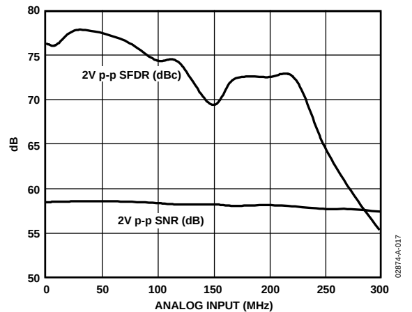
Figure 20. AD9215-65 SNR/SFDR vs. f_{\text{IN}} , A_{\text{IN}} = -0.5 \text{ dBFS} , f_{\text{SAMPLE}} = 65 \text{ MSPS}
