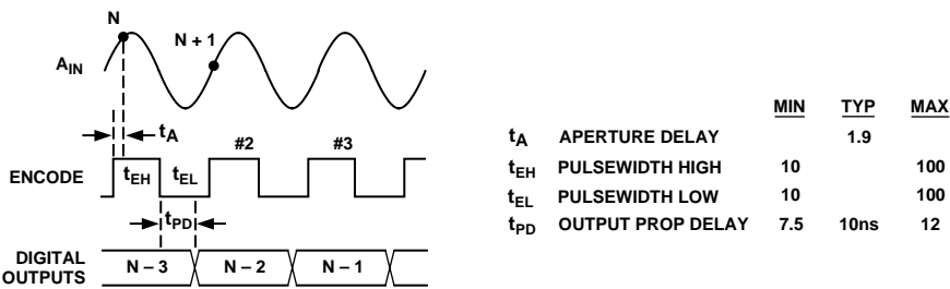
Figure 1. Timing Diagram
