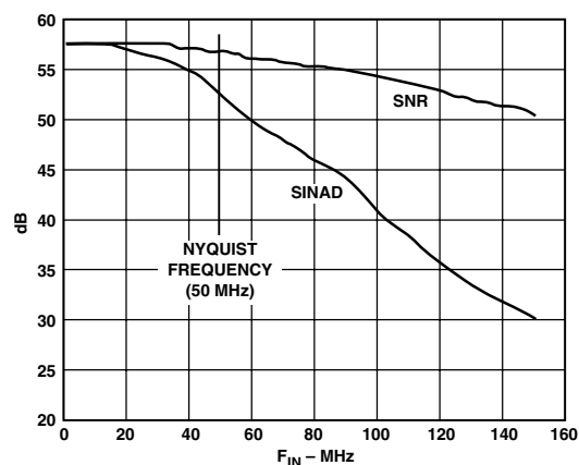
Figure 11. SNR vs. f_{IN} ; f_S = 100 MSPS
