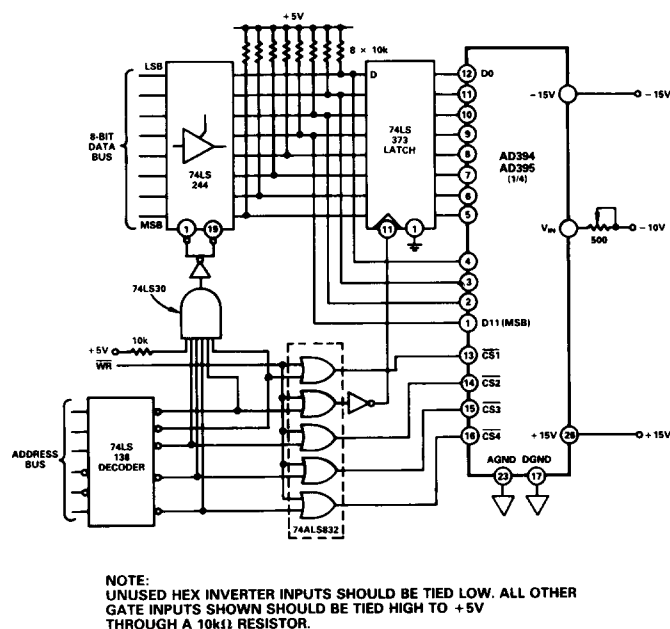
Figure 13. AD394, AD395 8-Bit Data Bus Interface
