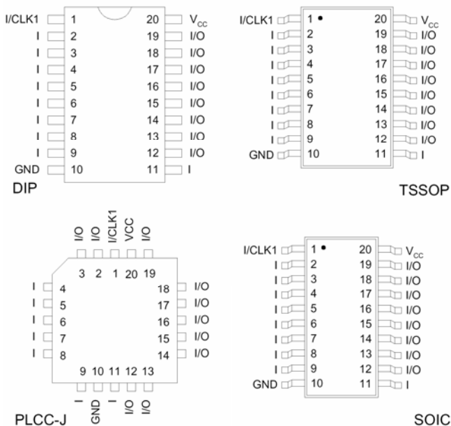
Figure 1 - Pin Configuration
