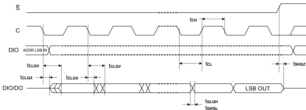
Figure 24. Output Timing
