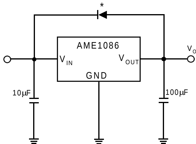
Figure 7 Regulator with reference
