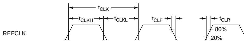
Figure 14. Clock Signal
