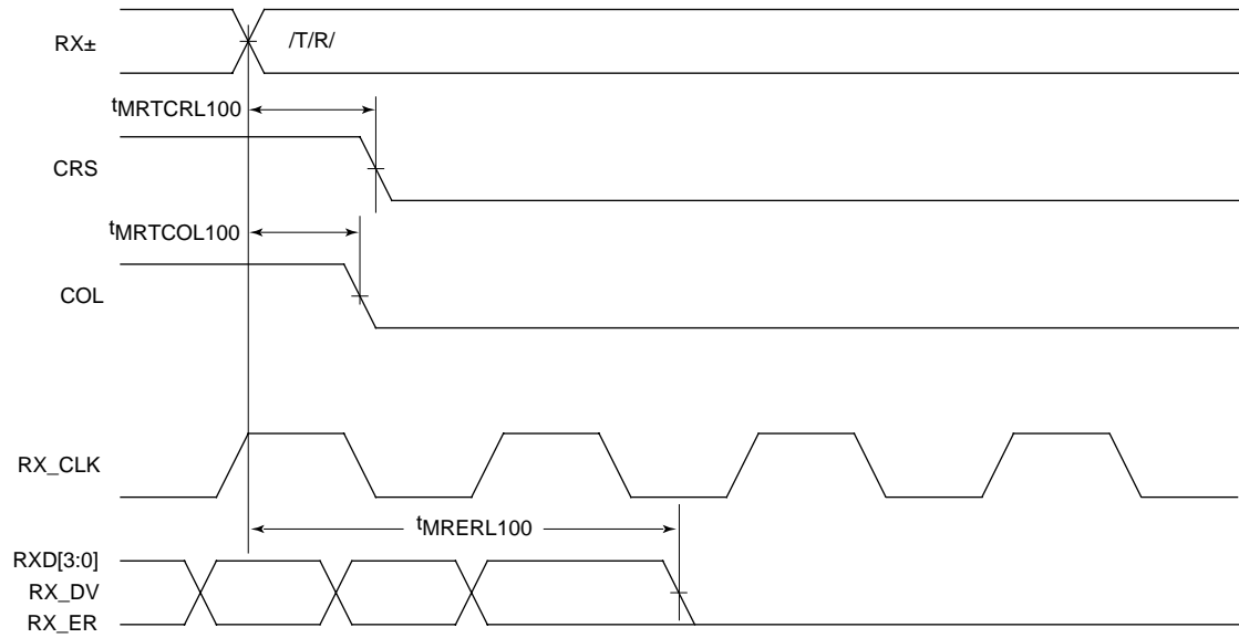
Figure 21. 100 Mbps MII Receive End of Packet Timing
