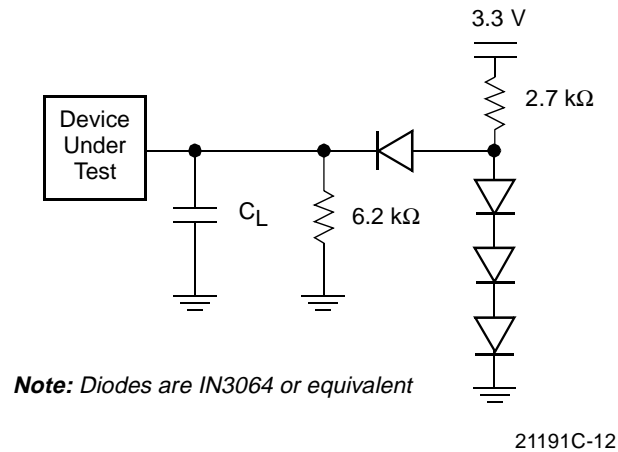
Figure 10. Test Setup
