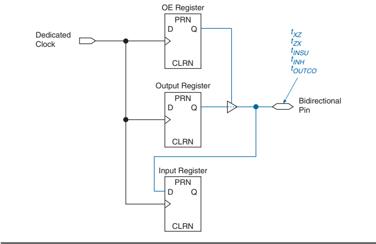
Figure 4–2. External Timing in Cyclone Devices
