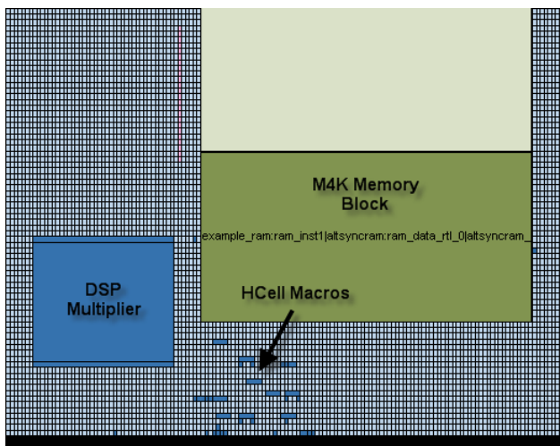
Figure 5–16. Close-Up View of Floorplan
