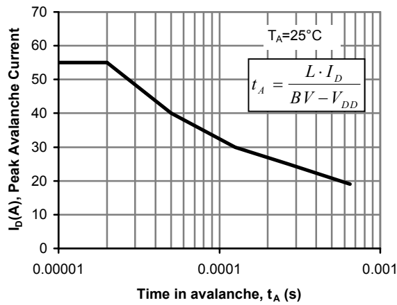
Figure 12: Avalanche capability
