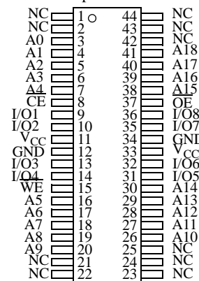
44-pin TSOP 2
