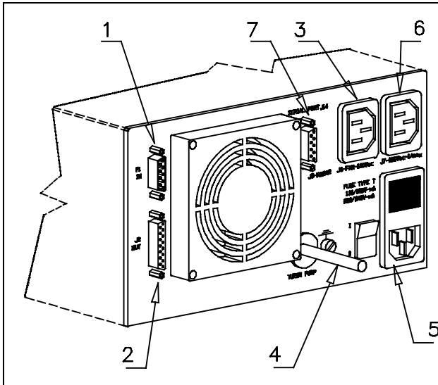
Controller 969-9445 and 969-9545 rear panel
