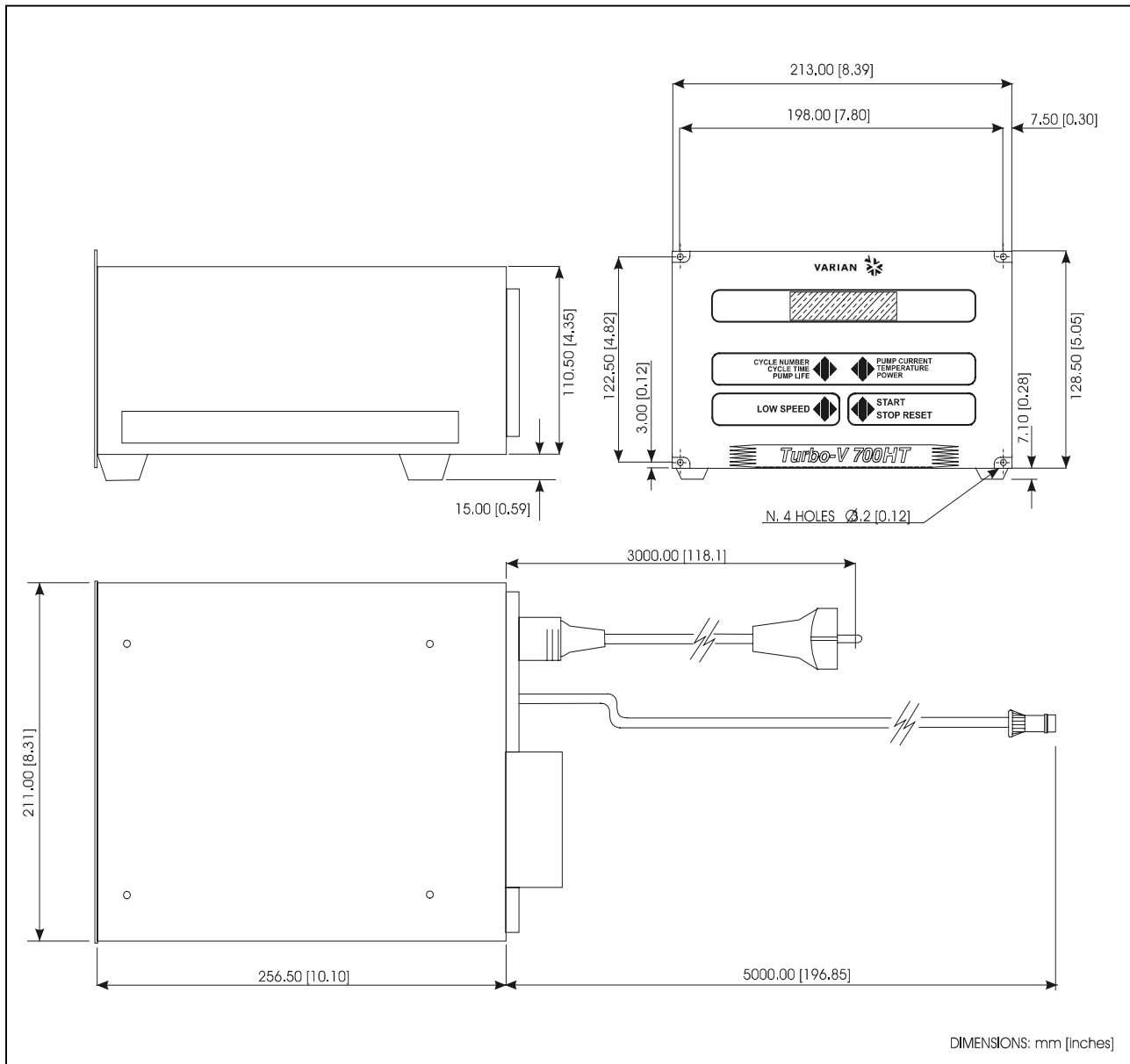
Controller models 969-9445 and 969-9545 outline
