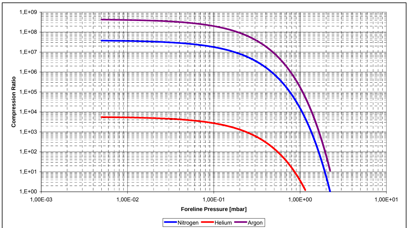
Compression Ratio Vs. Foreline Pressure
