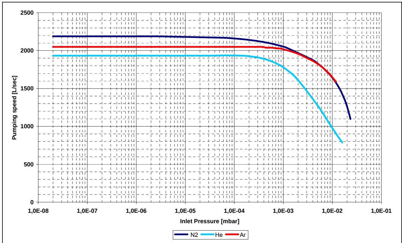
Typical Pumping Speed curves
