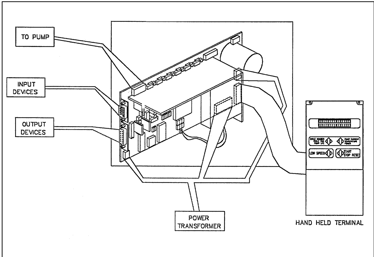
Controller interconnections
