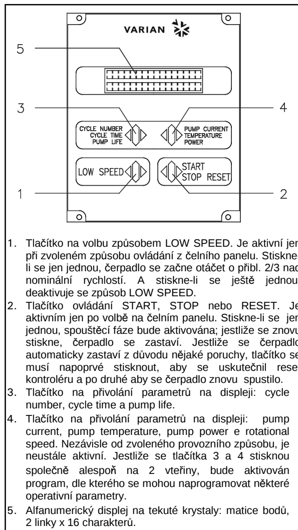
Čelní panel Hand Held Terminal
