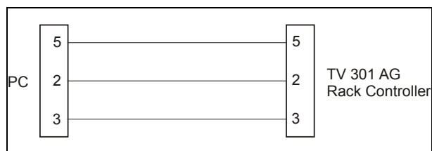
RS – 232 Connection
