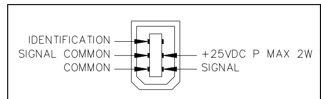
Gauge Connector
