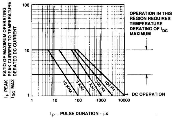
Figure 6. Maximum Tolerable Peak Current vs. Pulse Duration - HER Series.
