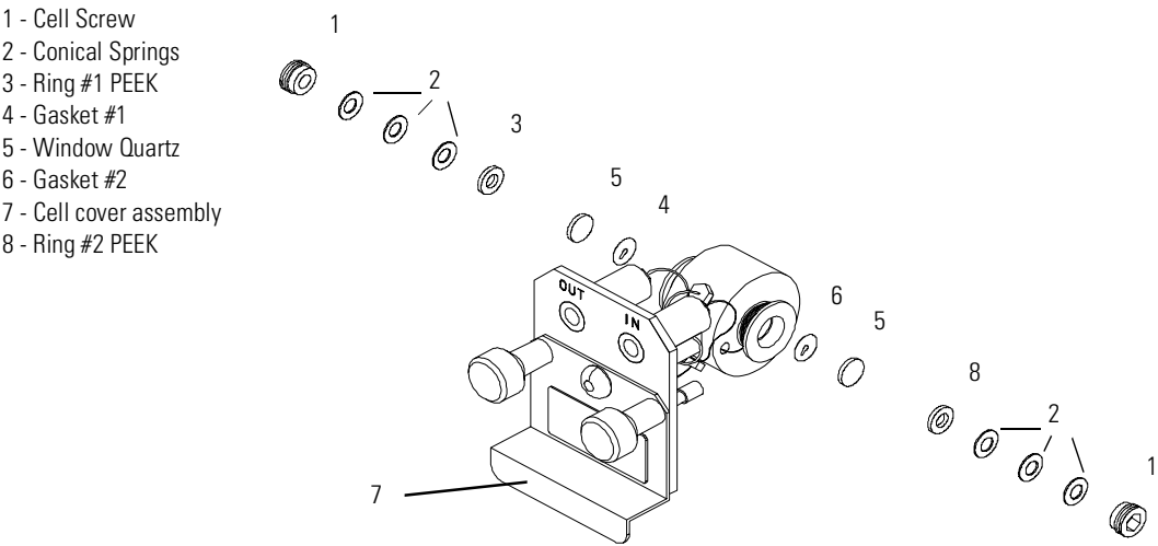
Figure 1 New Flow Cell
