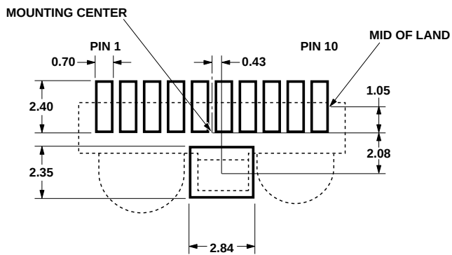
LAND PATTERN
