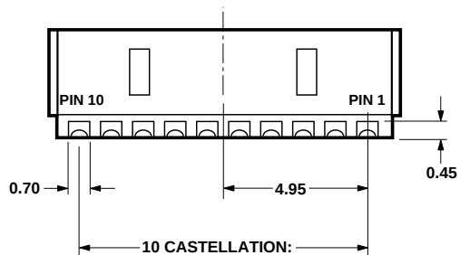
BACK VIEW
