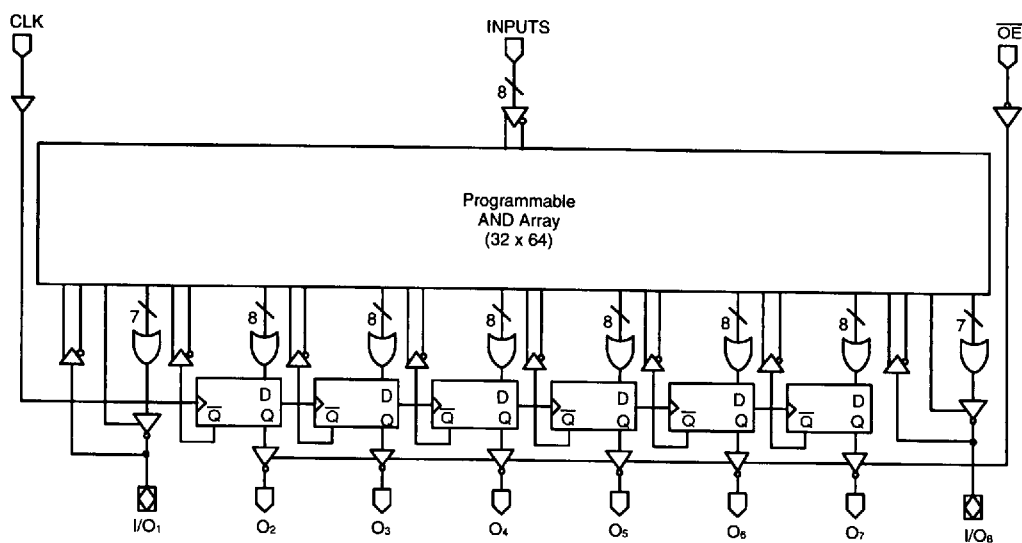
PAL16R6
