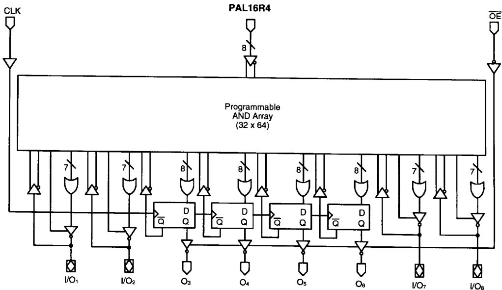
PAL16R4
