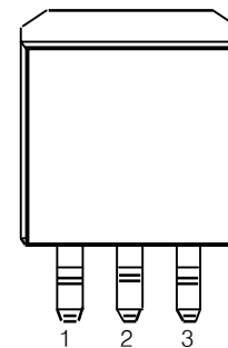
TO-263 (D2 PKG, FRONT VIEW)
