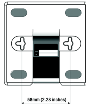
Figure 4-10: Measurement between Wall-Mount Slots
