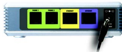
Figure 4-4: Connect Power
