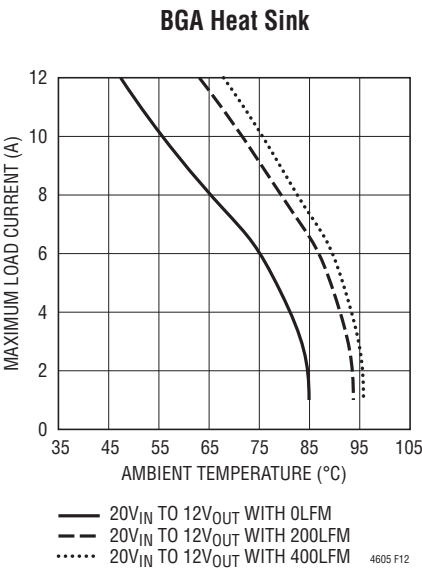
Figure 12. 20V IN to 12V OUT with Heatsink
