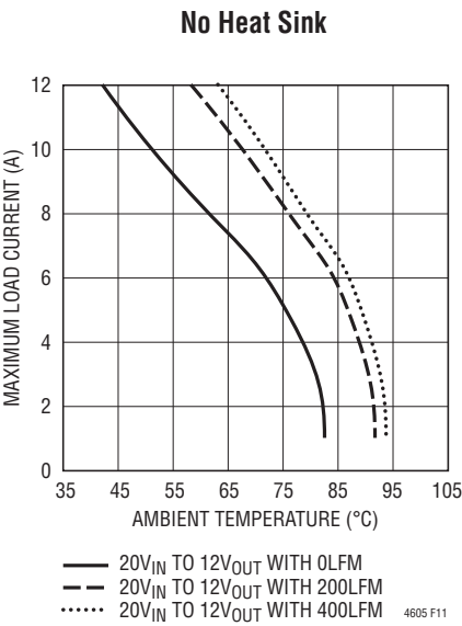
Figure 11. 20V IN to 12V OUT without Heatsink
