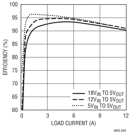
Efficiency vs Load Current 3.3μH Inductor (CCM)
