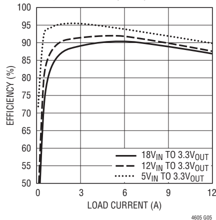
Efficiency vs Load Current 1.5μH Inductor (CCM)
