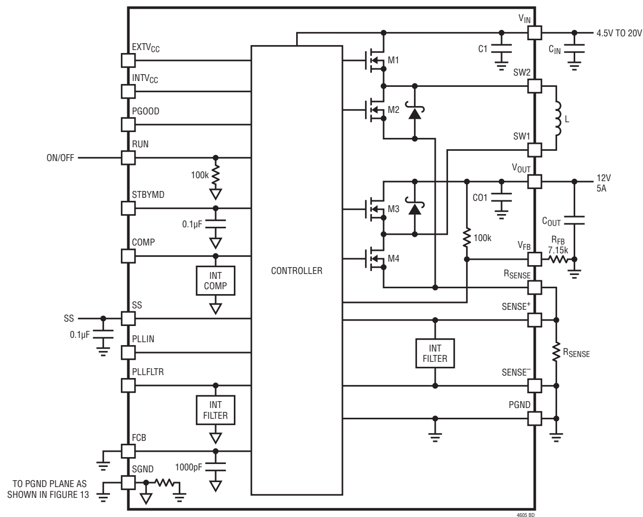
Figure 1. Simplified LTM4605 Block Diagram
