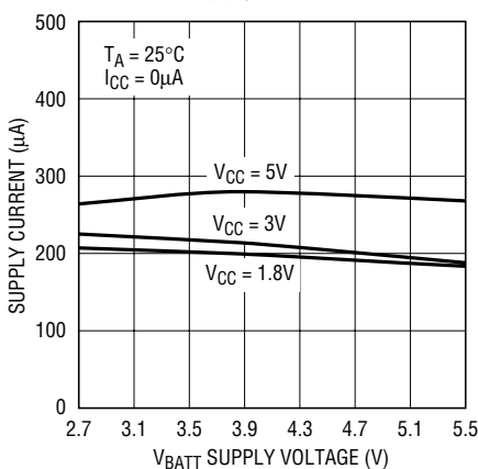
No Load Supply Current vs V_{\text{BATT}}
