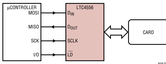
Figure 5. Microcontroller Interface
