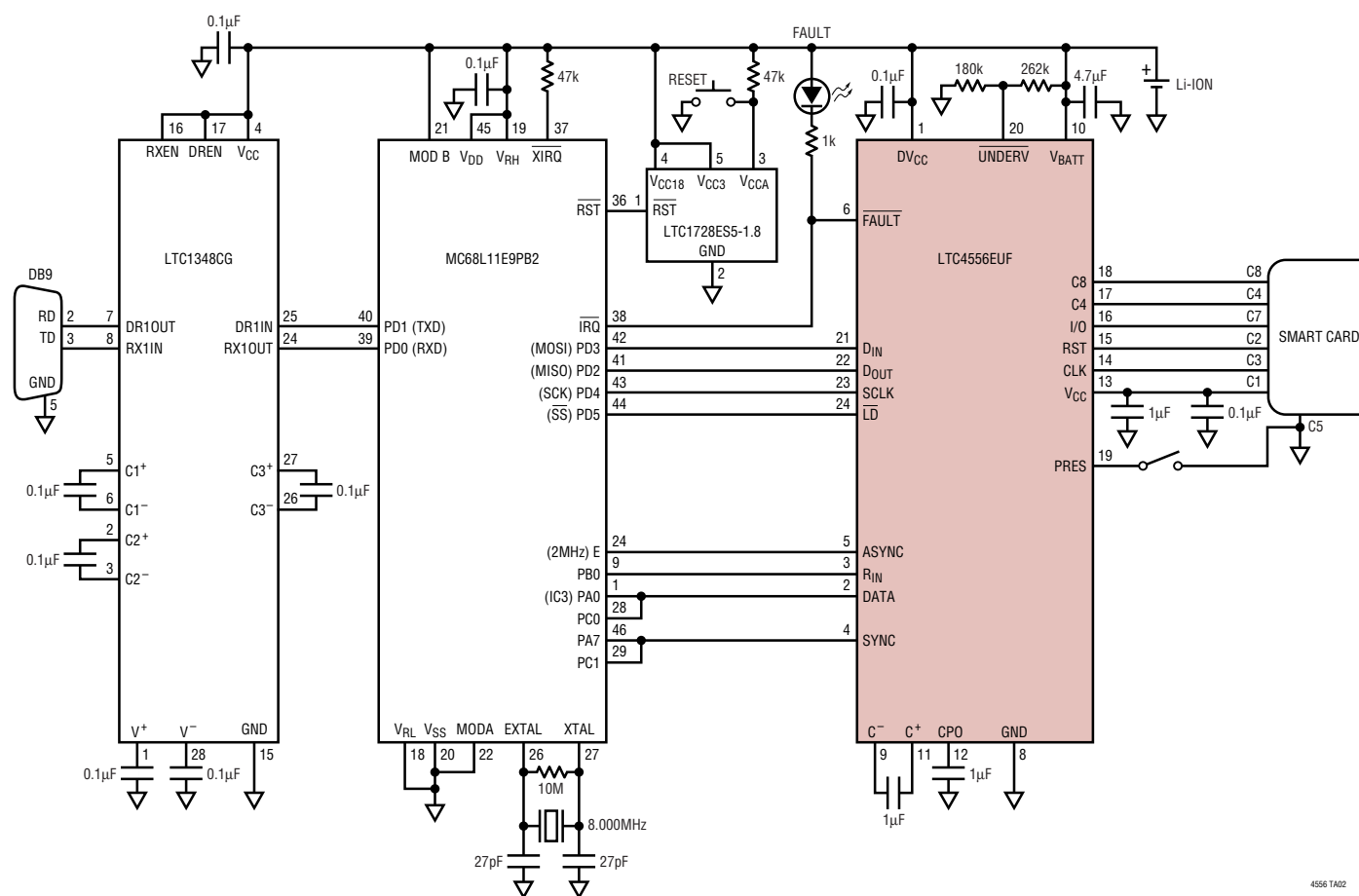
Battery-Powered RS232 to Smart Card Interface
