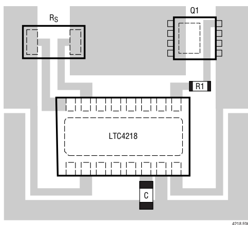
Figure 6. Recommended Layout
