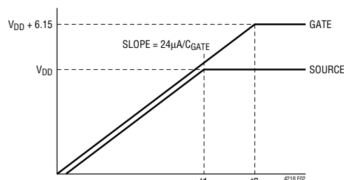
Figure 2. Supply Turn-On
