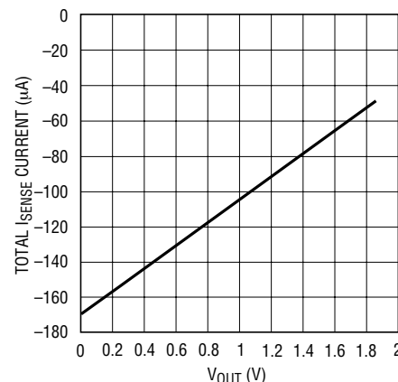
Total I_{SENSE} Current vs V_{OUT}
