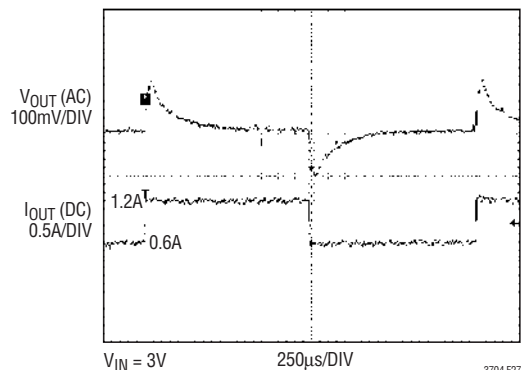
Figure 27. Load Step Response at 3V Input
