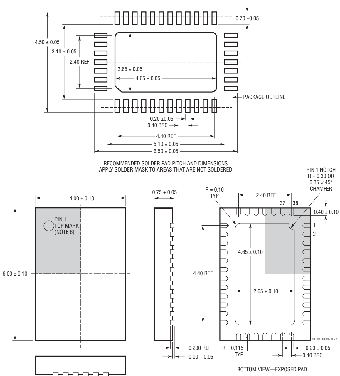
UFE Package 38-Lead Plastic QFN (4mm × 6mm) (Reference LTC DWG # 05-08-1750 Rev A)
