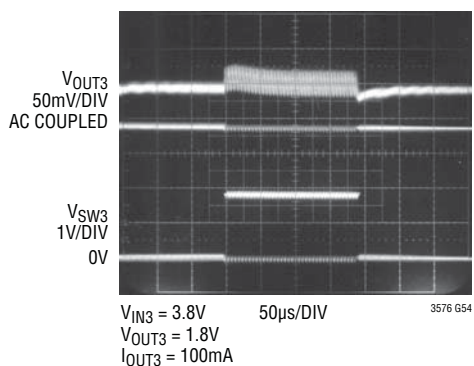
Switching Regulator Mode Transition, Pulse Skip-Burst Mode Operation-Pulse Skip
