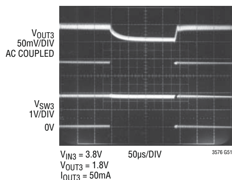
Switching Regulator Mode Transition, Pulse Skip-LDO-Pulse Skip
