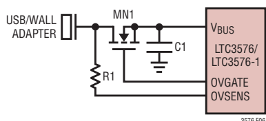
Figure 6. Overvoltage Protection
