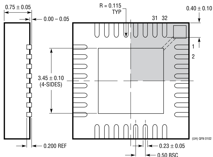
BOTTOM VIEW—EXPOSED PAD
