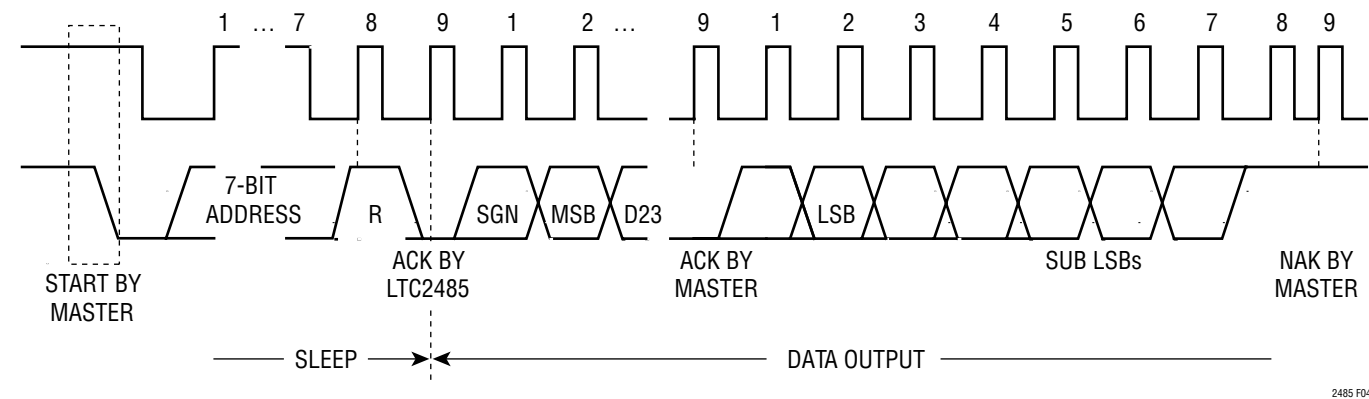
Figure 4. Timing Diagram for Reading from the LTC2485
