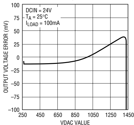
Voltage Accuracy
