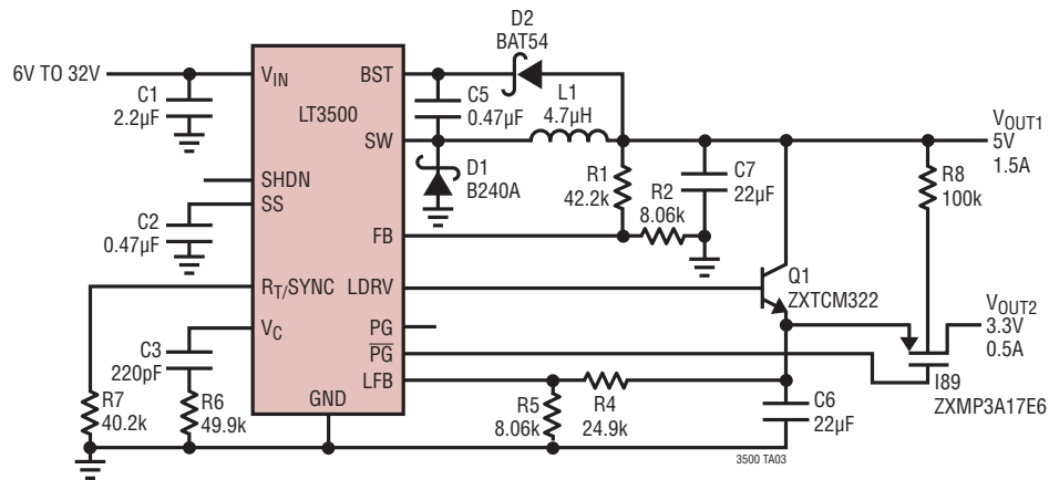
5V/1.5A, 3.3V/0.5A Step-Down with Output Disconnect
